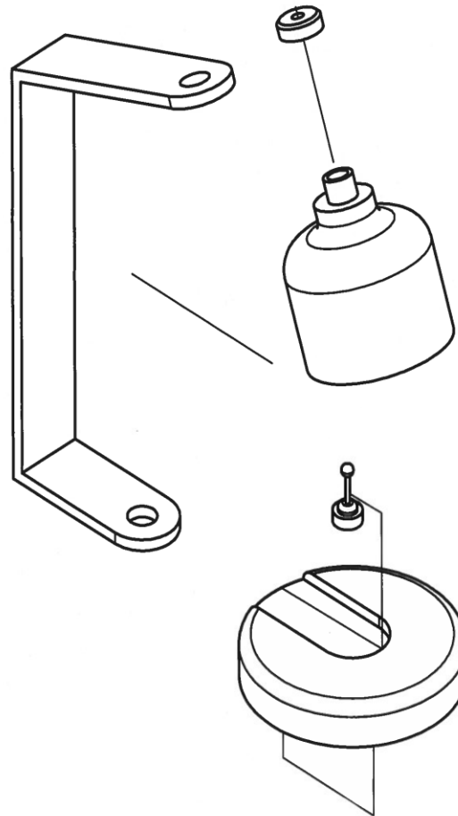
EXPLODED ISOMETRIC VIEW
