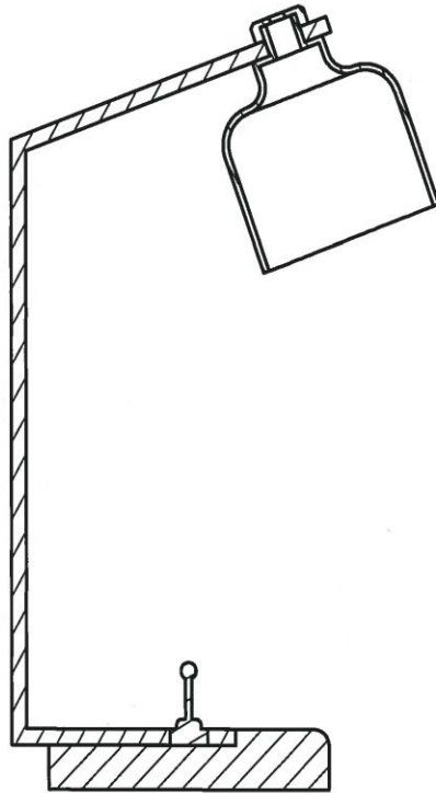
SECTIONAL FRONT ELEVATION
