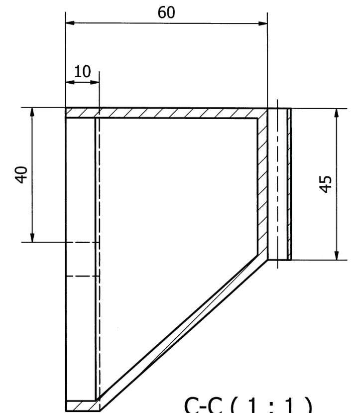
SECTIONAL END ELEVATION
