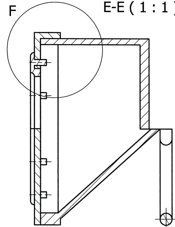
SECTIONAL END ELEVATION
